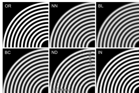
Figure 6: Original artificial image (OR) and 8X reduced/enlarged images (NN=Nearest Neighbor, BL=Bilinear interpolation, BC=Bicubic interpolation, ND=Nedi, IN=iNedi). The NEDI interpolation removes jagged contours, but introduces directional artifacts. iNedi modifications remove these effects.
