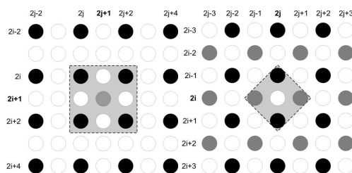
Figure 1: The two step NEDI interpolation. Original N \times N pixel are placed in a 2N-1 \times 2N-1 grid. Pixels at odd positions (2i+1, 2j+1) are then filled with the NEDI method (left) as weighted sums of the 4 diagonal neighbors. The remaining empty pixels are then filled in the same way after a 45^\circ rotation of the grid.
