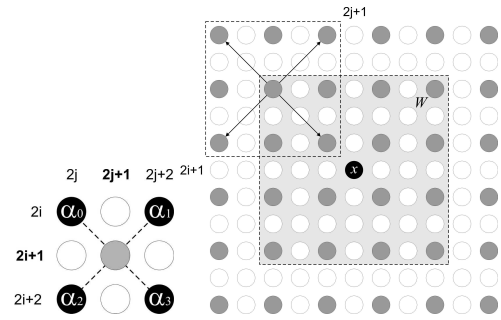
Figure 2: In the NEDI method, the four coefficient used to compute the interpolated value (left) are computed assuming that in a squared window around the point each pixel of the low resolution image is related through the same coefficients to its 4 closest neighbors.
