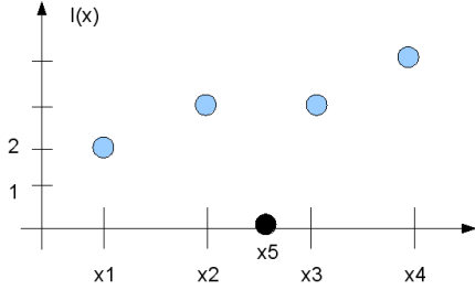
Figure 3: A simple 1D interpolation example showing that an exact constant covariance interpolation may create completely wrong results. Assuming that each pixel at the low resolution can be obtained as a weighted sum of the two neighbors and assuming weights locally constant, we obtain the black pixel as the one interpolating the profile in x_5 .
